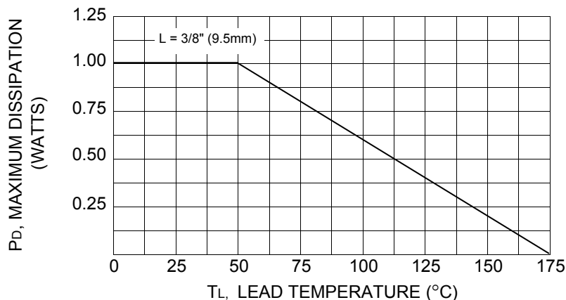
Fig. 1 POWER TEMPERATURE DERATING CURVE
